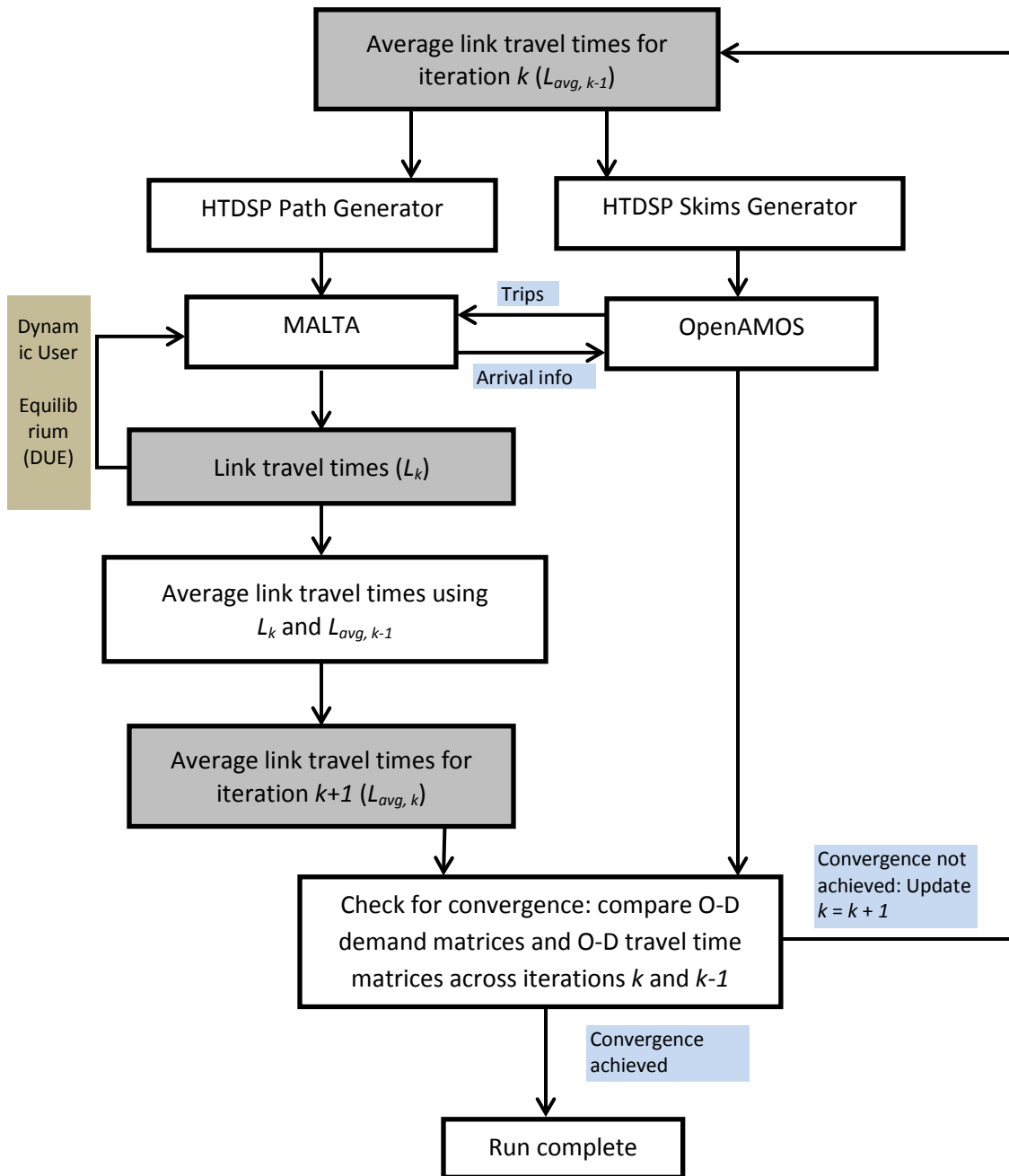
Figure 1: Operational overview of the integration between MALTA and OpenAMOS
